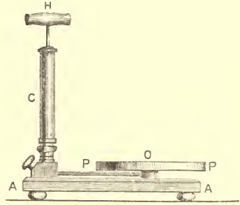
FIG. 1.—Simplest Form of Air Pump.
